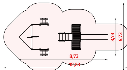
Top view with impact area
