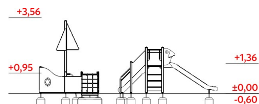
General view of device
